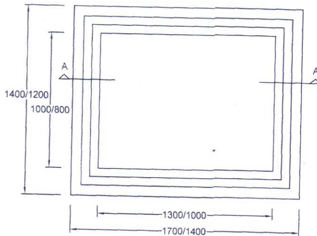
PLAN OF TRANSFORMER FOUNDATION
